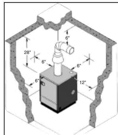
Minimum clearance dimensions
